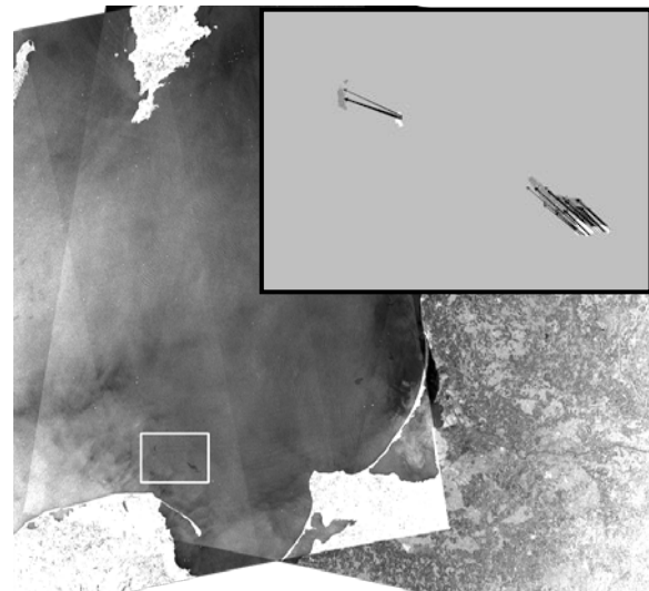
Figure 1. Composite of two ASAR images of the southeastern Baltic Sea acquired on May 15, 2005. The white square north of the Bay of Gdansk denotes the (82.5 km × 60 km) part of the images used for the correlation analysis, whose results are inserted on the upper right.
