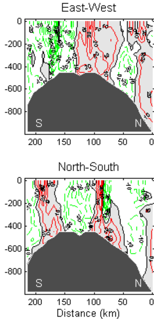
Figure 5: g) East-west component of the velocity distribution across the Iceland Faroe Ridge (cm/s). Red lines represent the eastward and green lines represent the westward flow.
