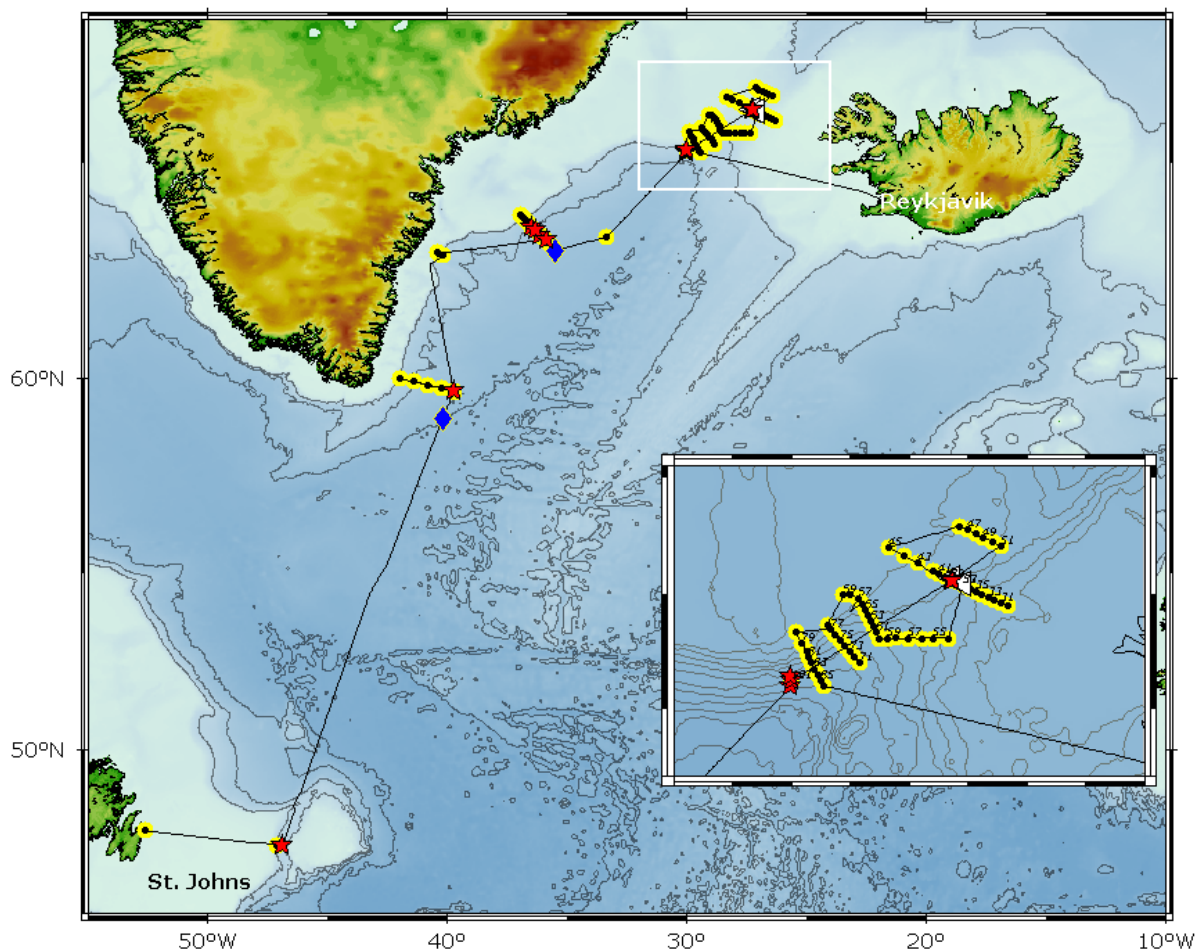
RV METEOR M85/2 cruise track from St. Johns to Reykjavik. Yellow dots indicate CTD+ casts, blue symbols Argo float deployments, red stars mooring operations, white triangle PIES deployments.
